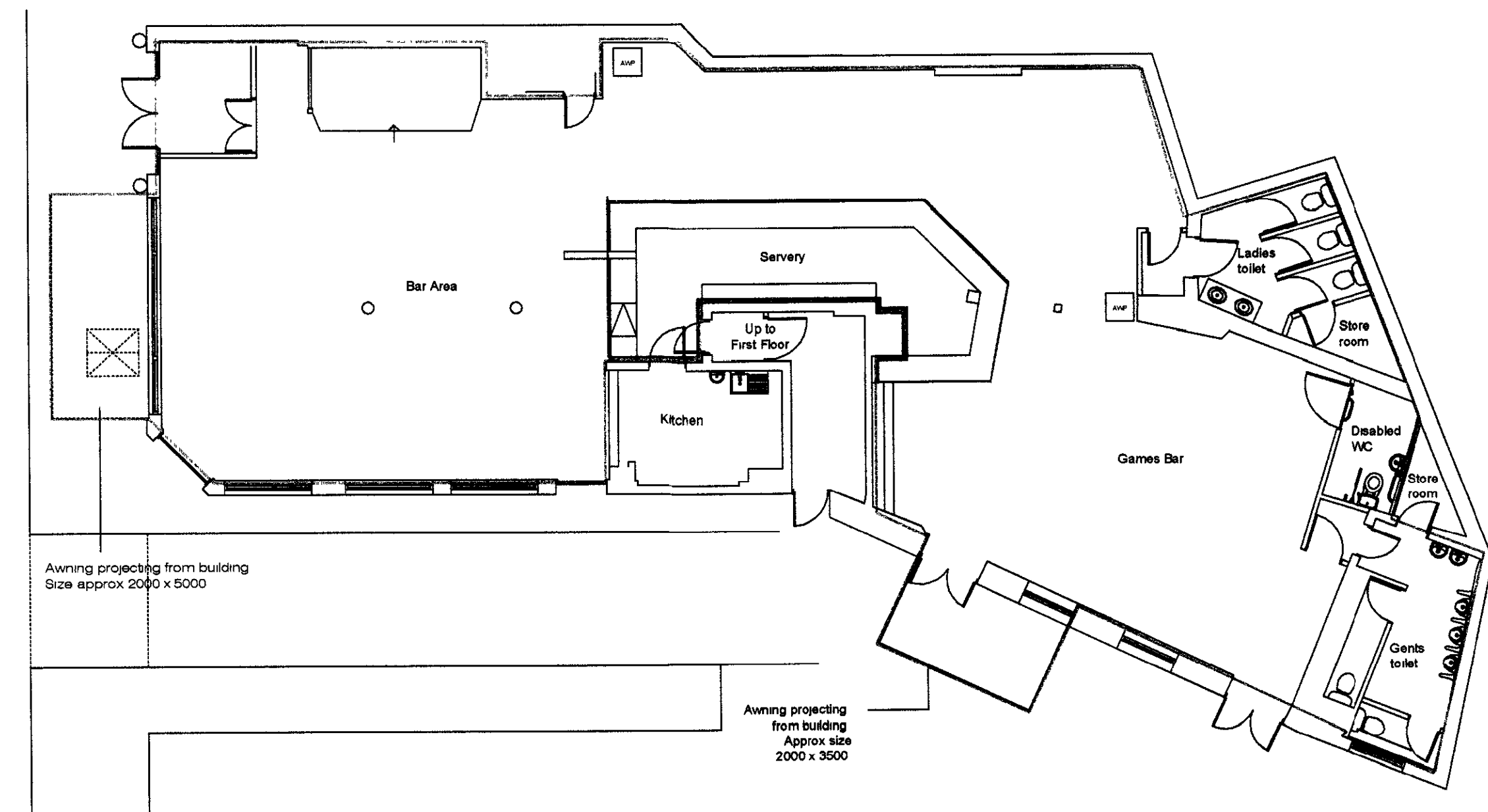
PROPOSED PLAN
